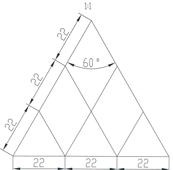
DETAIL DRAWING OF TUBE PITCH 孔距详图
