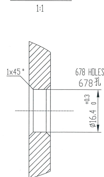
DETAIL DRAWING OF DRILLING 钻孔详图
